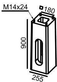
CONCRETE FOUNDATION B-50
